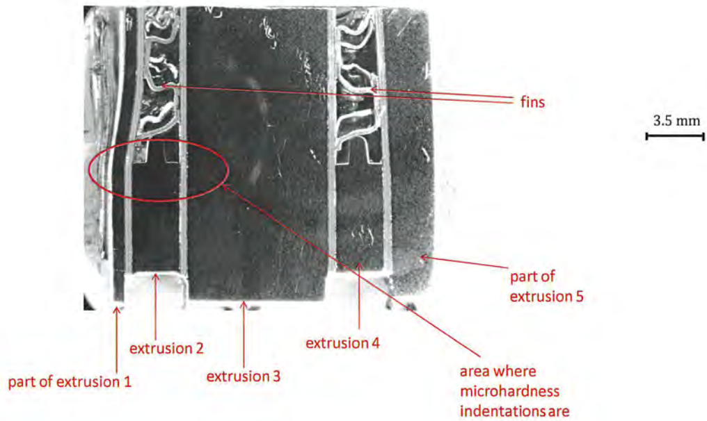
Figure 1. Low-magnification view of the cross-section of the manufactured aluminum alloy part (sample) showing various elements identified.
