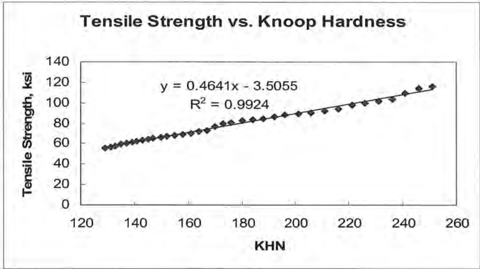
Figure 5. Tensile strength – Knoop hardness number (500 gr) correlation obtained from Wilson (Instron) Desk Chart 60 (1992).
