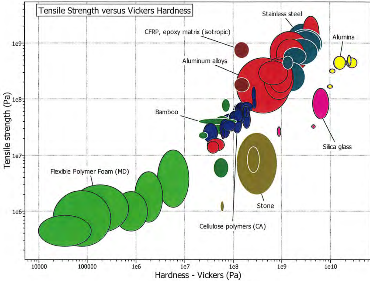
Figure 6. CES plot of tensile strength vs. Vickers hardness (obtained using Cambridge Engineering Selector EduPack 2012).
